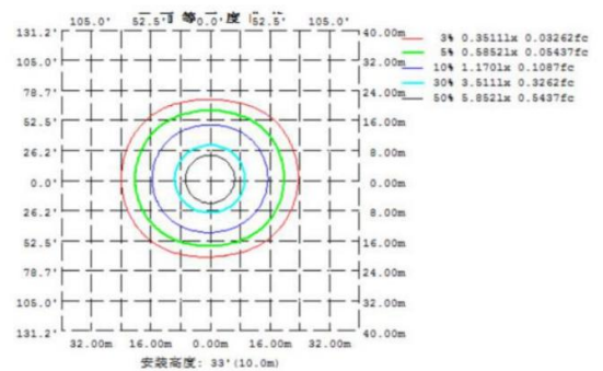
Isolux Plot
