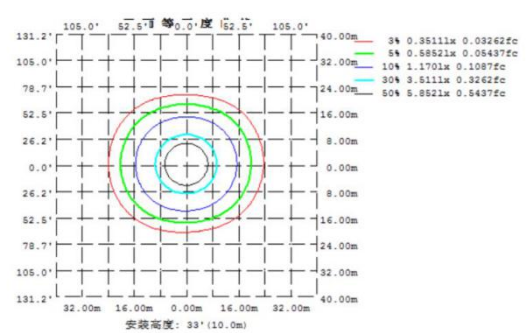
Isolux Plot
